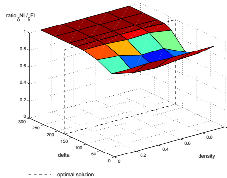
Fig. 10. The figure represents how ratio \delta NI/\delta FI is varying with \delta and CSP density for weighted CSPs.
