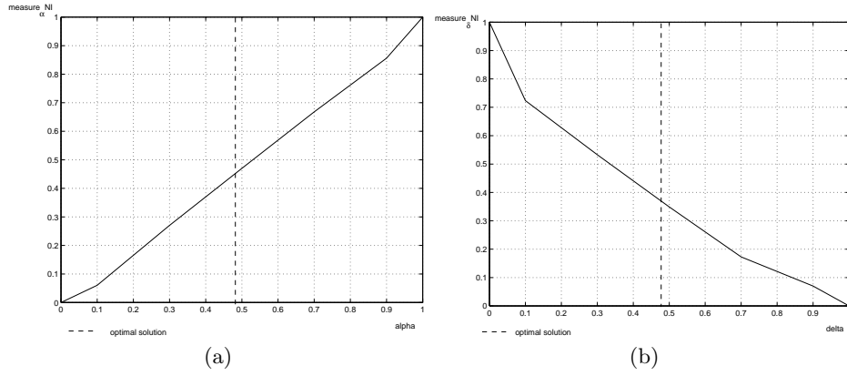
Fig. 3. A statistical measure of the number of NI of \alpha/\delta interchangeability for Fuzzy CSP with uniform weight distribution, for sets of problems with 10 variables and 10 values domains (Figure (a) for \alpha and Figure (b) for \delta ).
